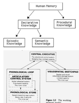
Figure 2.2 The working memory model
