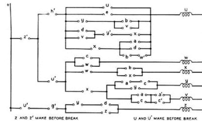
Figure 34. Combination-lock circuit
